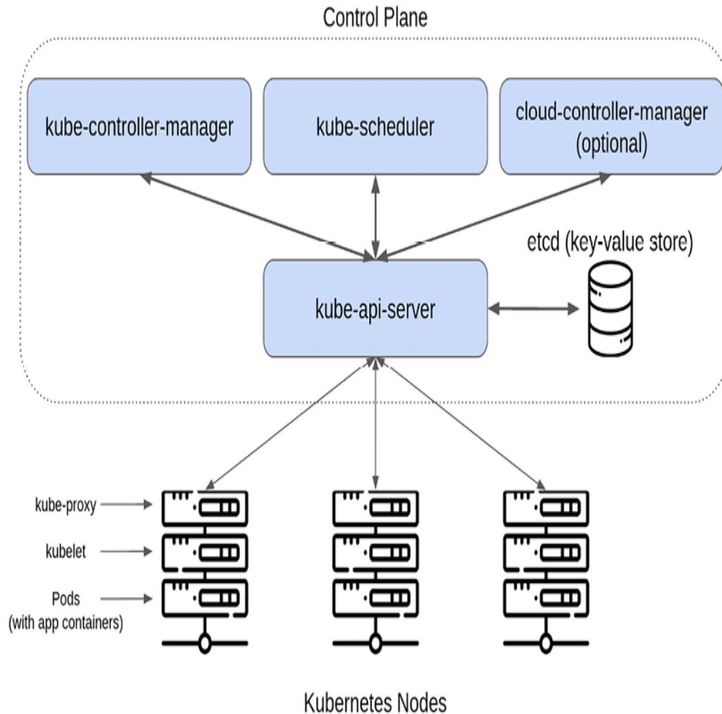
Figure 6.15: The K8s architecture.
