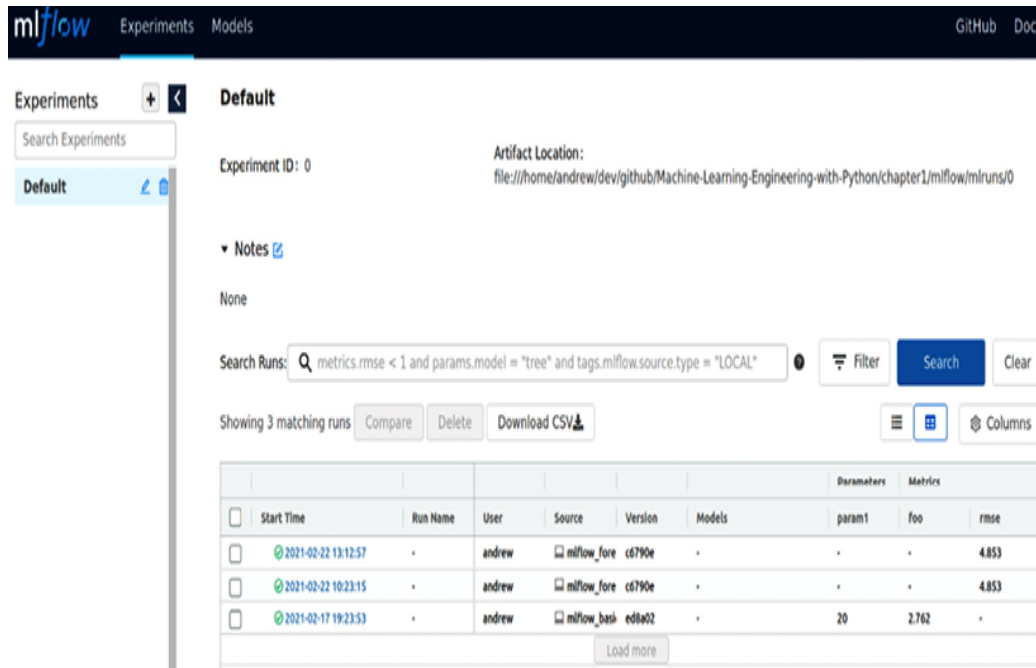
Figure 2.11: The MLflow tracking server UI with some forecasting runs.
