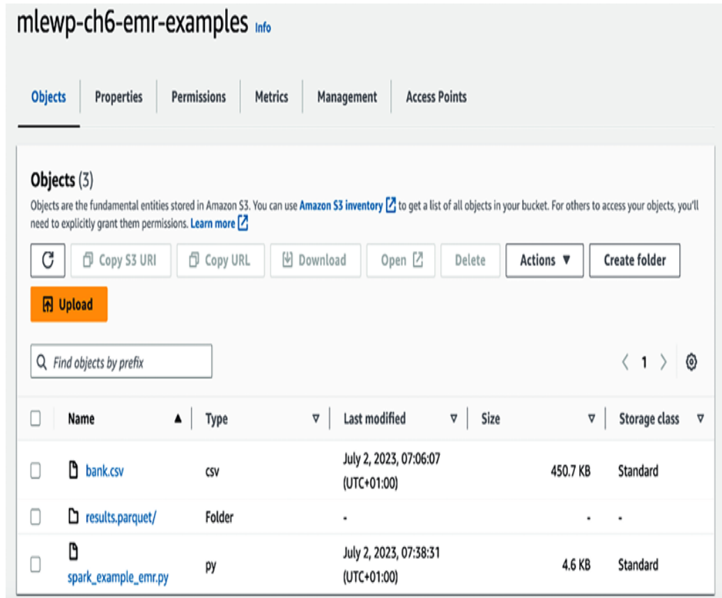
Figure 6.13: Successful creation of the results.parquet file upon submission of the EMR script.
