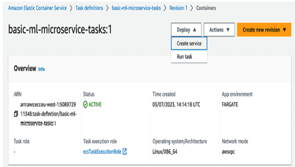
Figure 5.15: Selecting the Create service option for the task definition we have just created in the previous steps.
