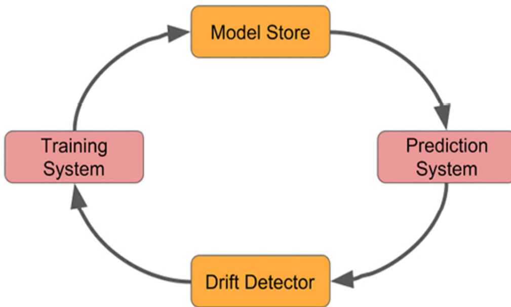
Figure 3.1: The components of the model factory.
