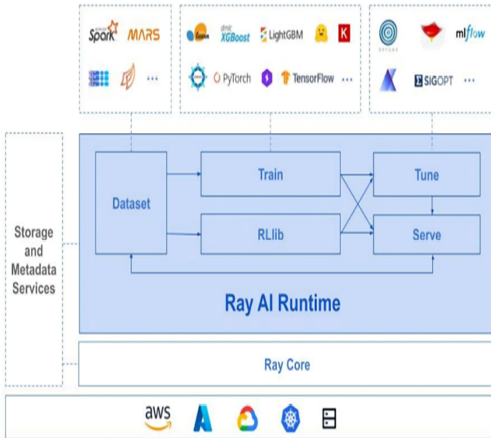
Figure 6.16: The Ray AI runtime, from a presentation by Jules Damji from Anyscale: https://microsites.databricks.com/sites/default/files/2022-07/Scaling%20AI%20Workloads%20with%20the%20Ray%20Ecosystem.pdf . Reproduced with permission.
