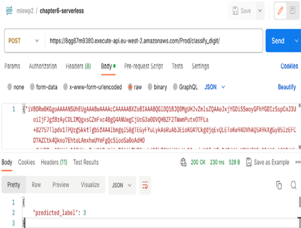
Figure 6.14: Calling our serverless ML endpoint with Postman. This uses an encoded example image as the body of the request that is provided with the SAM XGBoost ML API template.
