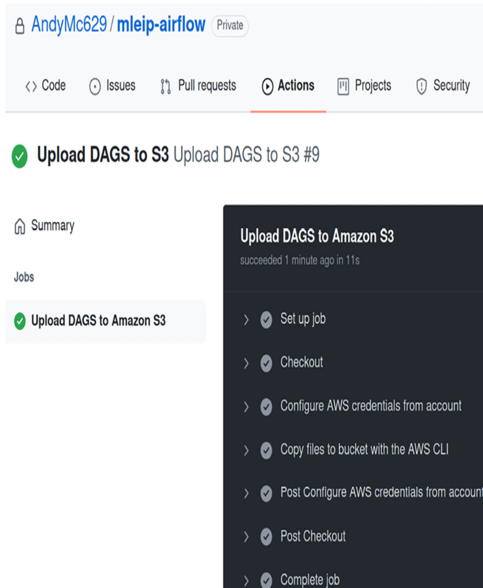
Figure 5.35: A successful CI/CD process run via GitHub Actions and using the AWS CLI.
