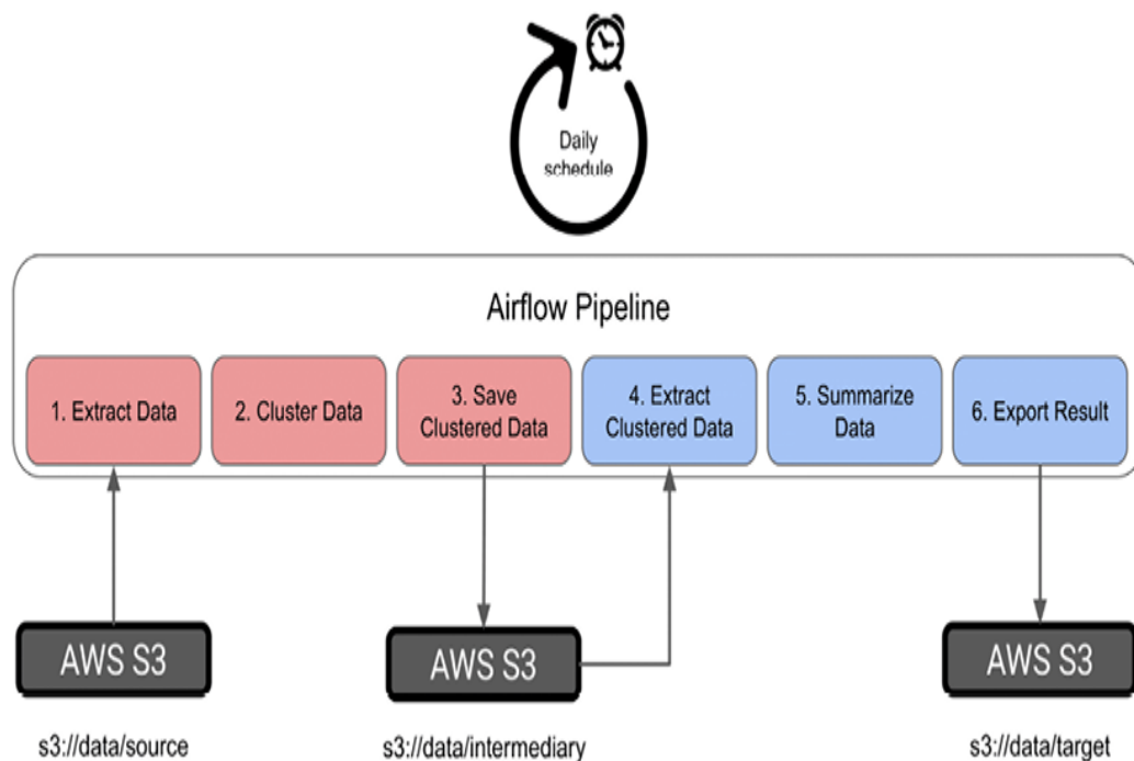
Figure 9.4: High-level design for the ETML clustering and summarization system. Steps 1–3 of the overall pipelines are the clustering steps and 4–6 are the summarization steps.
