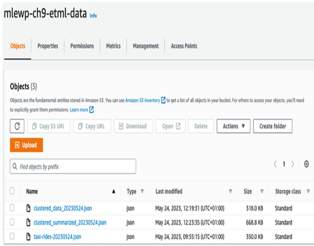
Figure 9.9: The successful run of the DAG creates the intermediate and final JSON files.
