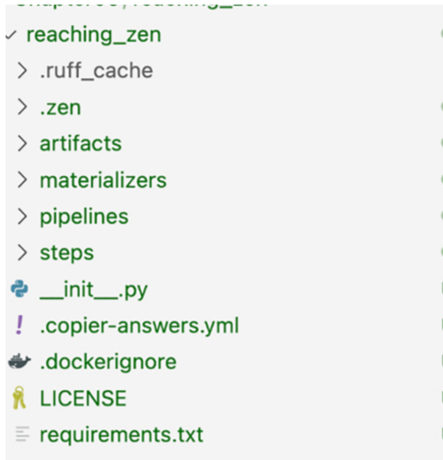
Figure 5.39: File and folder structure generated after using the ZenML template generation wizard.
