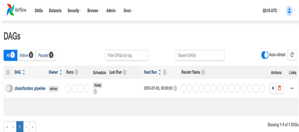
Figure 5.33: The Airflow UI accessed via the AWS MWAA service. This view shows the classification DAG that we wrote earlier in the example.
