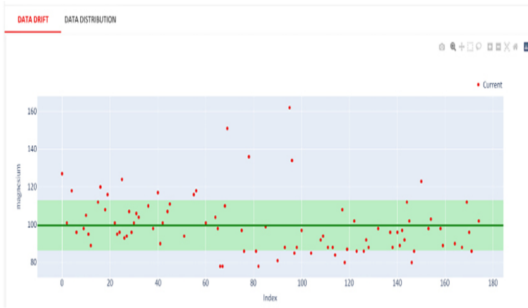
Figure 3.9: The automatically generated data drift plot when you drill down in the Evidently report for the Wine features.
