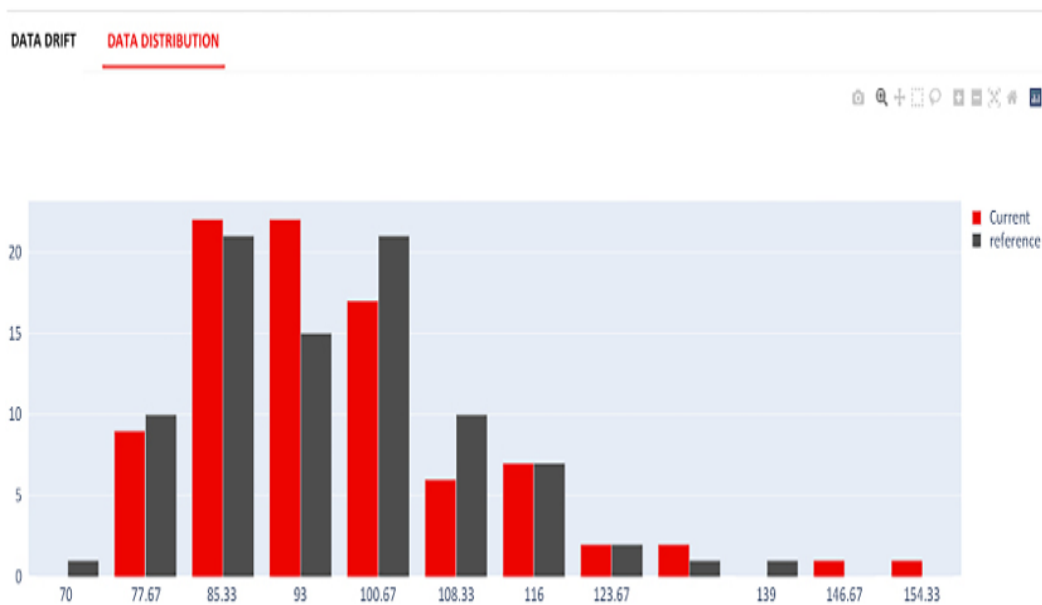
Figure 3.10: The automatically generated histogram showing the distribution of the feature when you drill down in the Evidently report for the Wine feature set.
