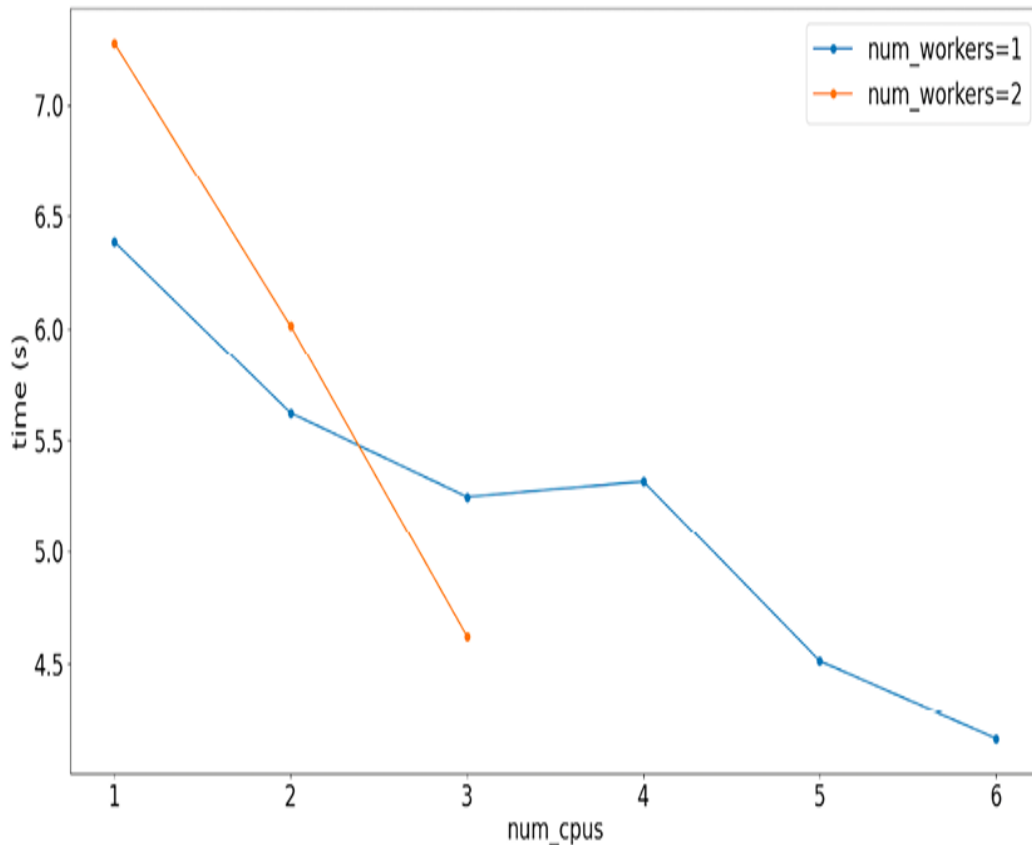
Figure 6.20: A few experiments show how changing the number of workers and CPUs available per worker results in different XGBoost training times on the author’s laptop (an 8 core Macbook Pro).
