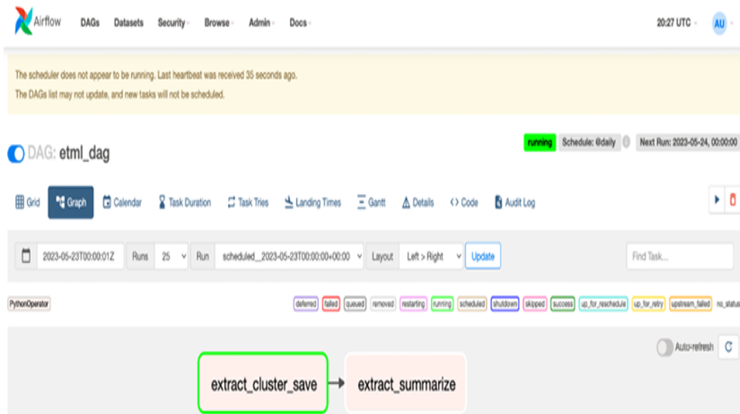
Figure 9.8: The ETML DAG in the Airflow UI.
