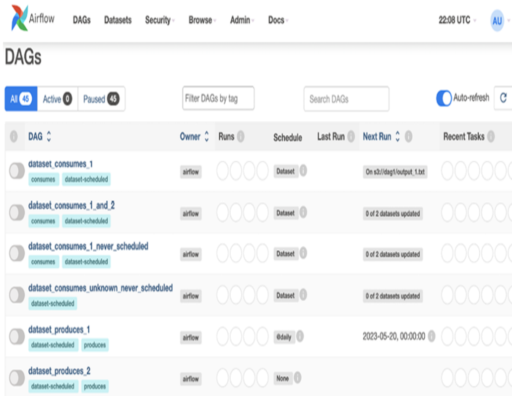
Figure 9.3: The landing page after logging in to the standalone Airflow instance. The page has been populated with a series of example DAGs.
