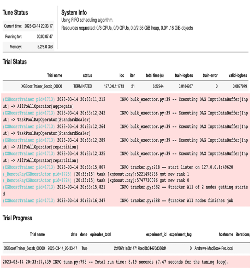
Figure 6.19: Output from parallel training of an XGBoost model using Ray.
