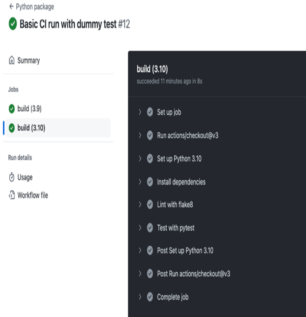
Figure 2.15: The GitHub Actions run steps as shown on the GitHub UI.
