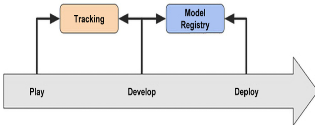
Figure 3.12: How the MLflow Tracking and Model Registry functionalities can help us progress through the different stages of the ML development process.
