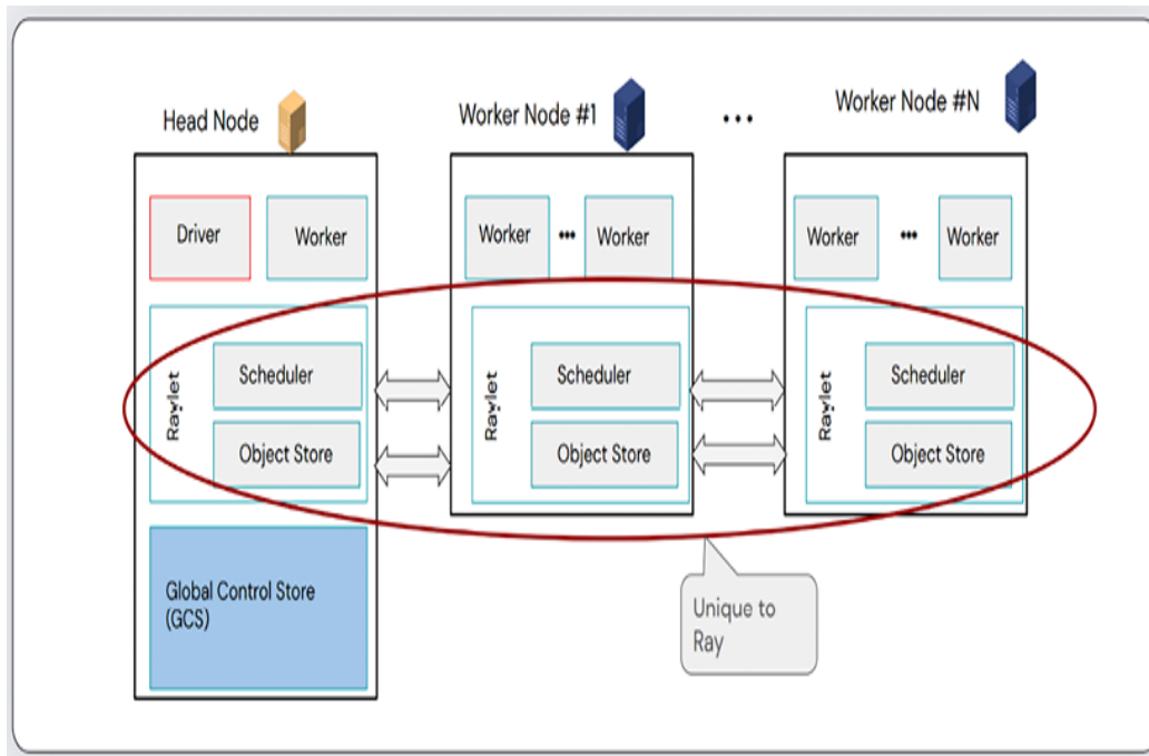
Figure 6.17: The Ray architecture including the Raylet scheduler. From a presentation by Jules Damji: https://microsites.databricks.com/sites/default/files/2022-07/Scaling%20AI%20Workloads%20with%20the%20Ray%20Ecosystem.pdf . Reproduced with permission.
